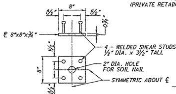
BASE P DETAIL
