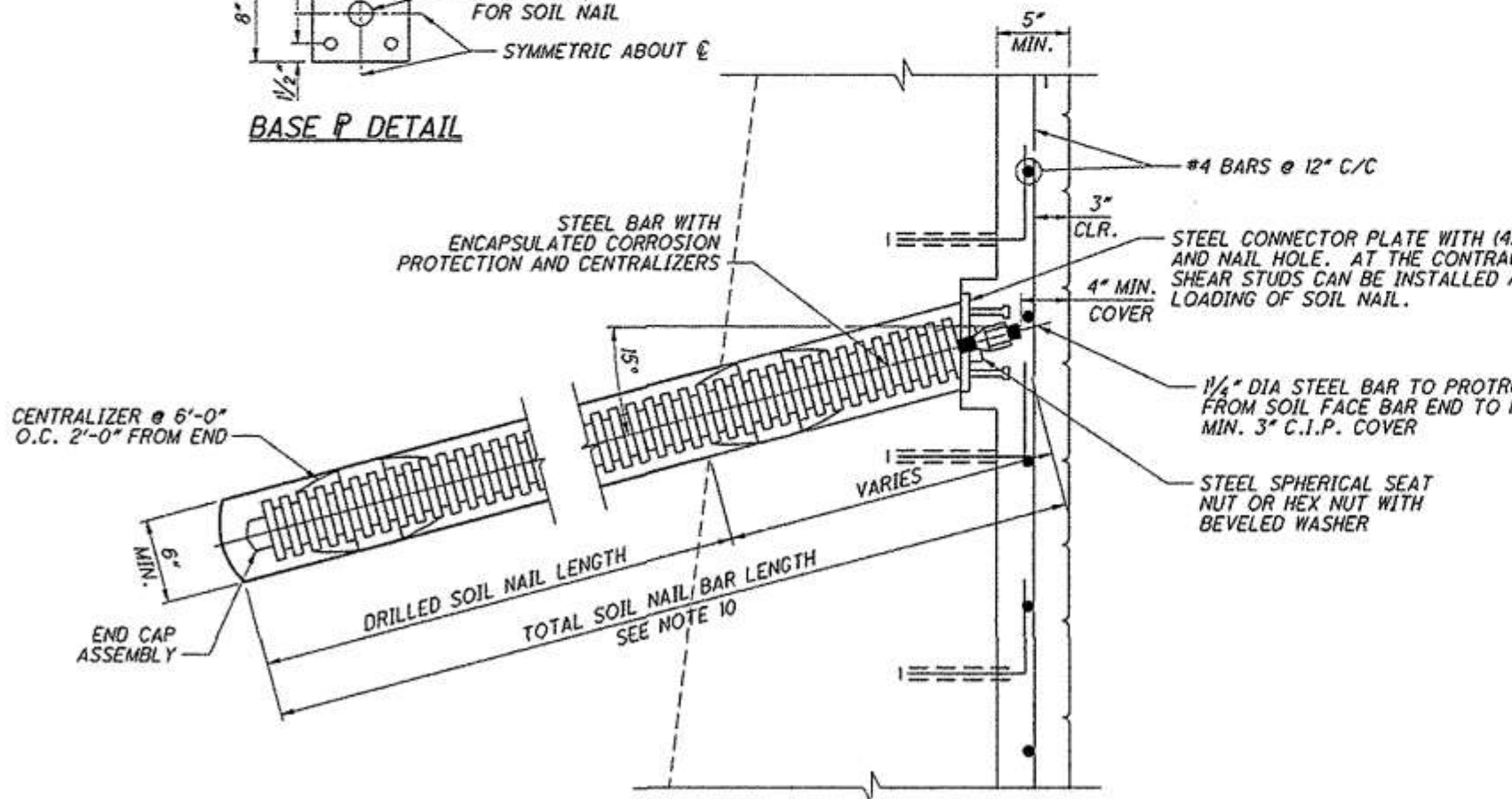
TYPICAL SOIL NAIL SECTION
